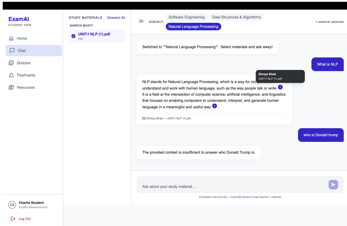
Figure 9.4: RAG chat — per-session material scope, numbered citations with teacher/file tooltip, and grounded refusal of an off-corpus question.
