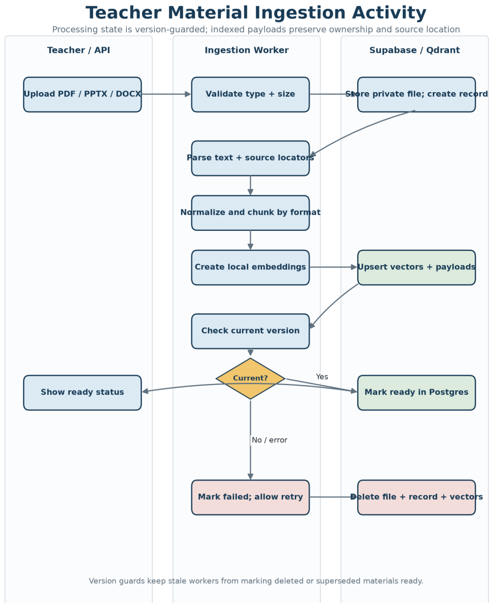
Figure 8.5: Material ingestion activity
