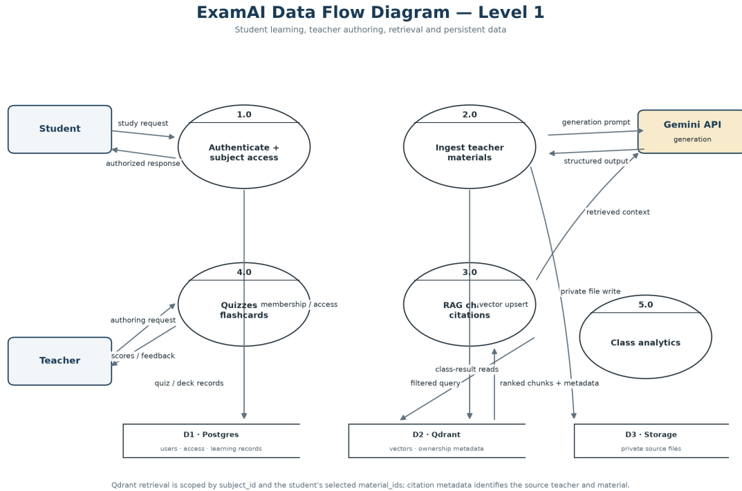
Figure 8.6.2: Level 1 DFD
