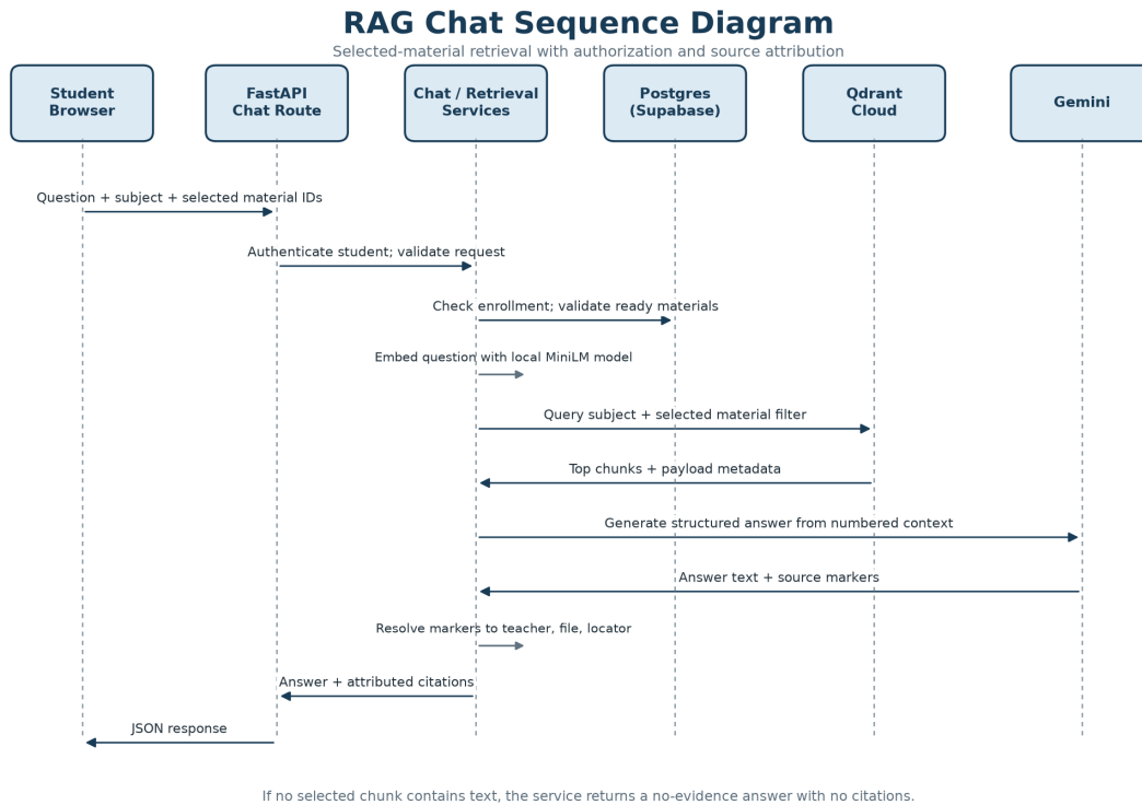
Figure 8.4: RAG chat sequence
