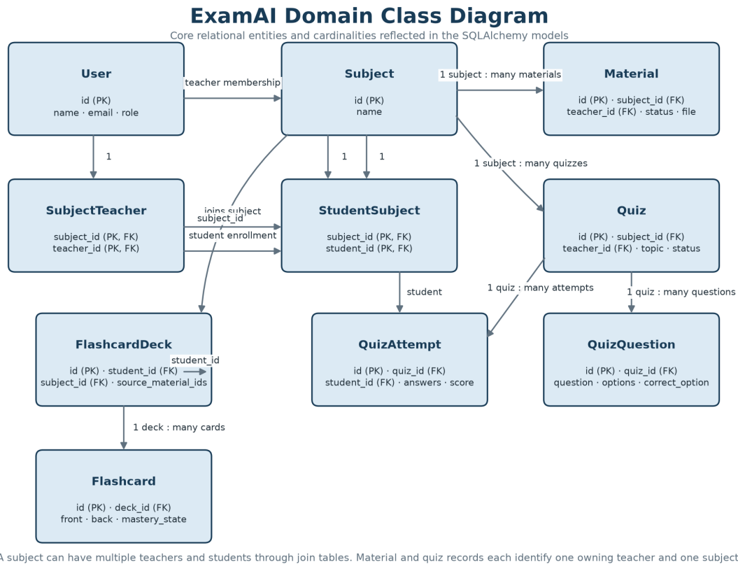
Figure 8.2: Class diagram
