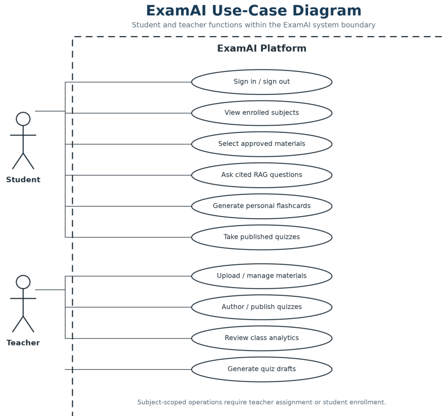
Figure 8.3: Use-case diagram
